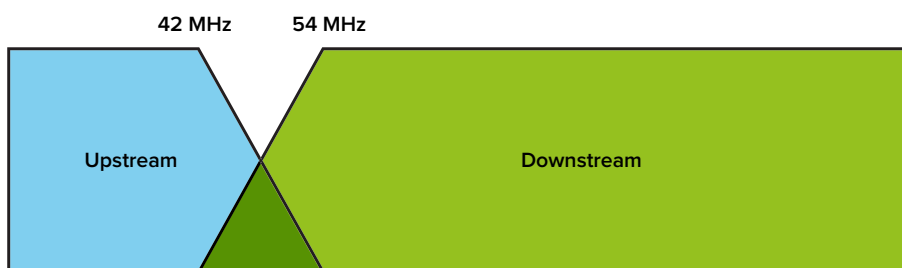
Figure 3_The frequency split with crossover area
