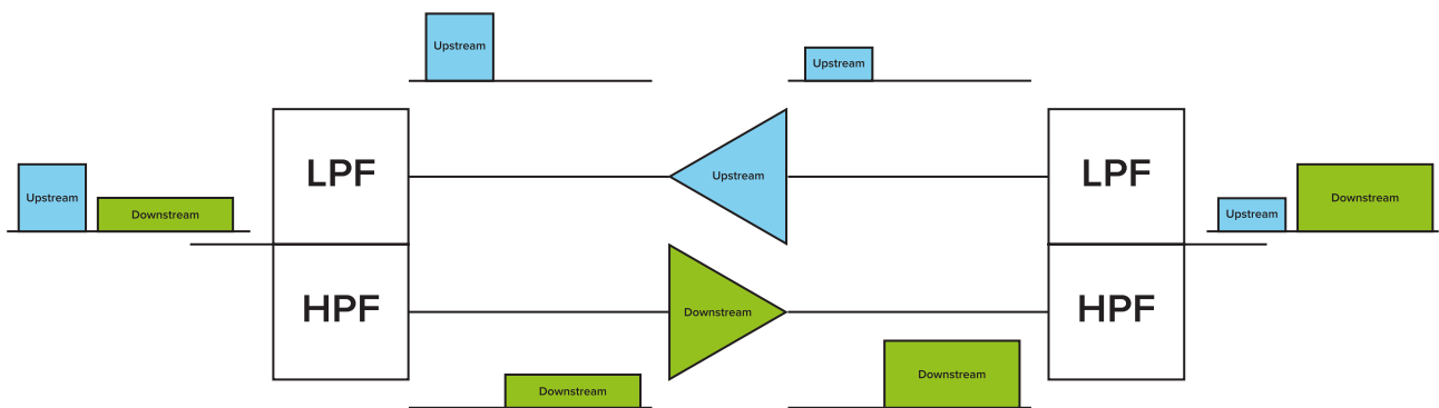
Figure 2_An amplifier with diplex filters
