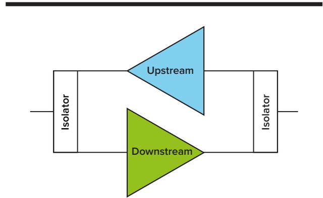
Figure 4 _The diplex-free amplifier
